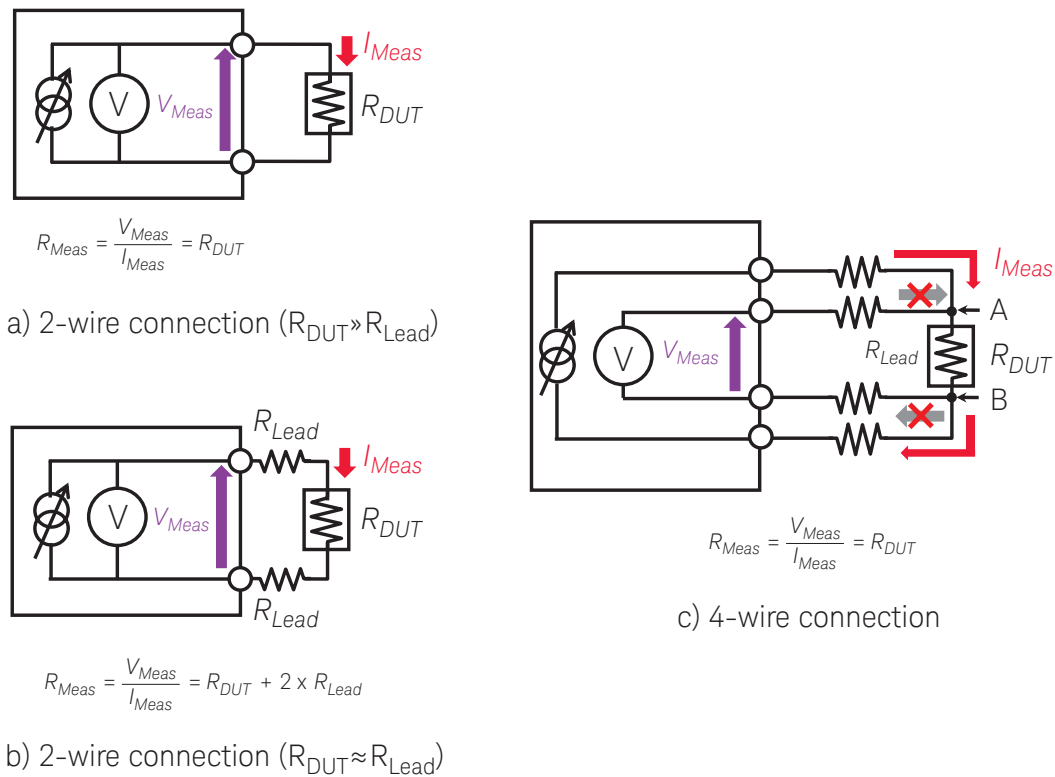
Figure 13. A 4-wire connection eliminates measurement errors caused by residual lead resistance
